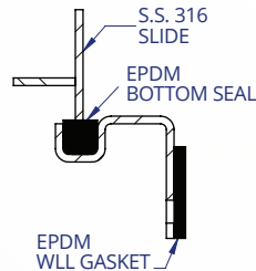
BOTTOM SEAL
